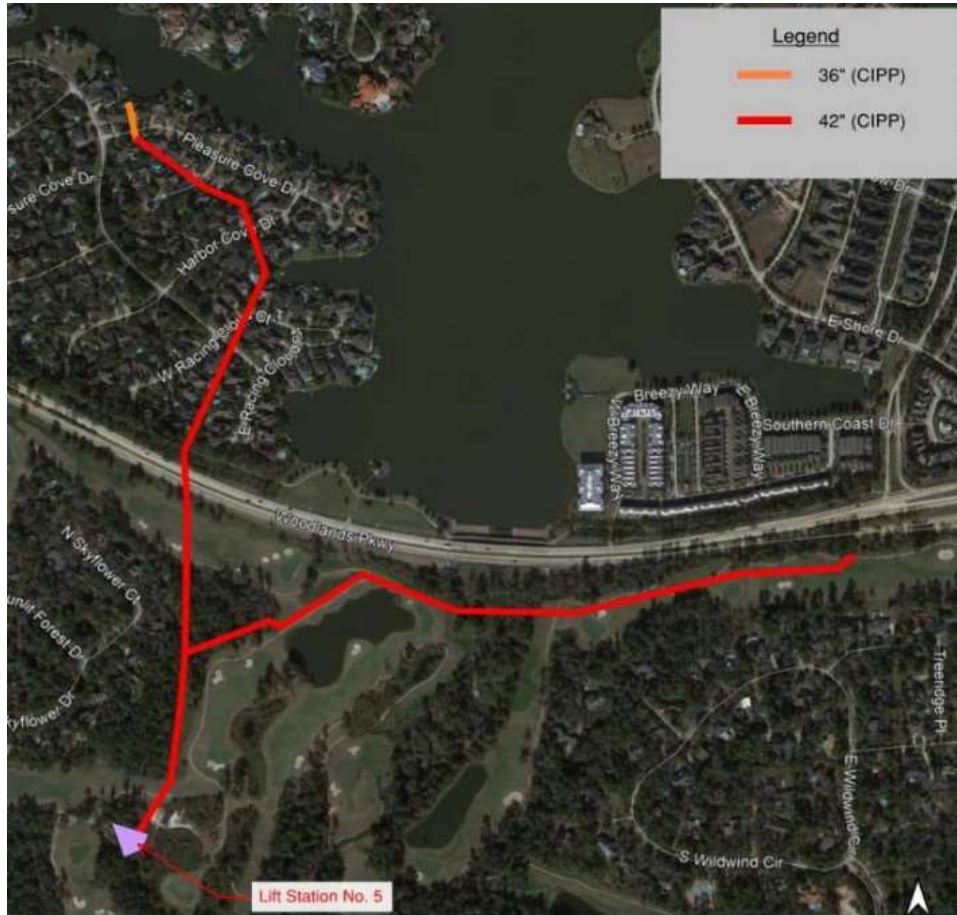
Figure 1: Aging Gravity Main Infrastructure of Interest
