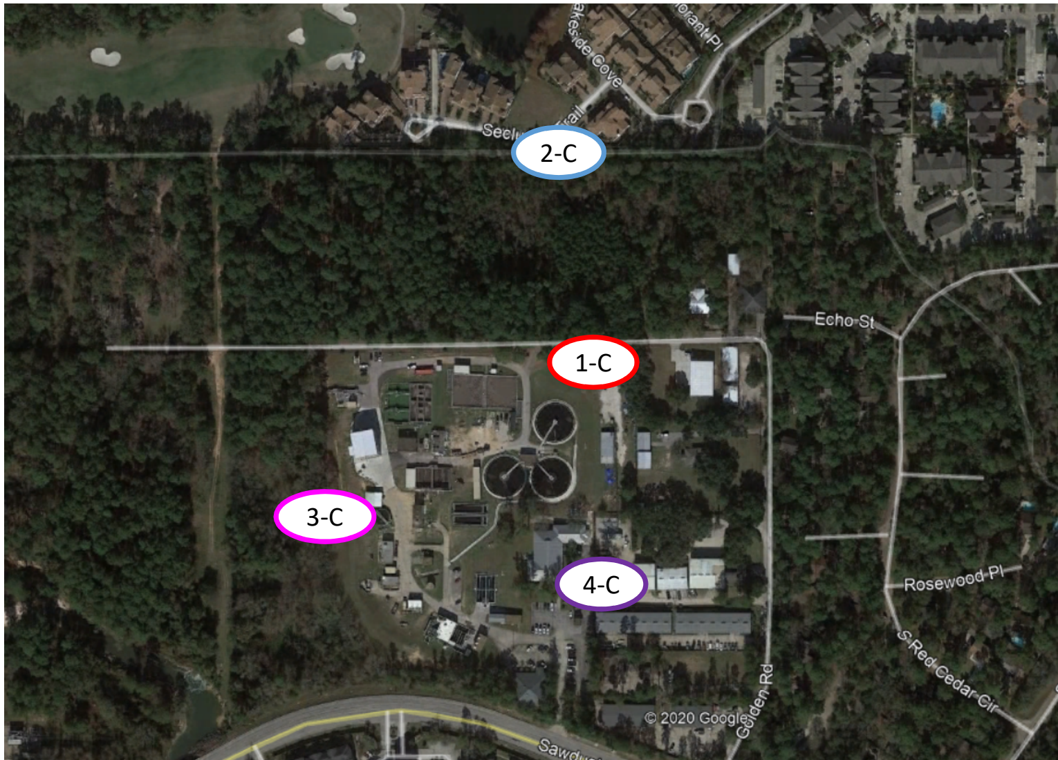
WWTF NO. 1 ODOR MONITOR LOCATIONS – WEEK 3 (C)
